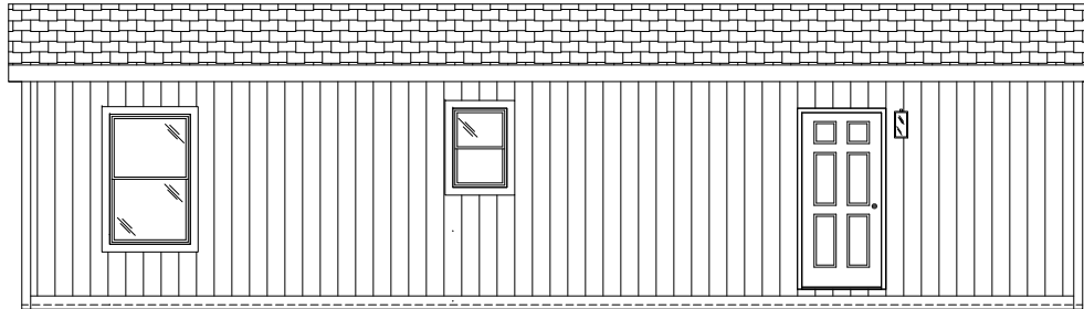
FRONT SIDEWALL
