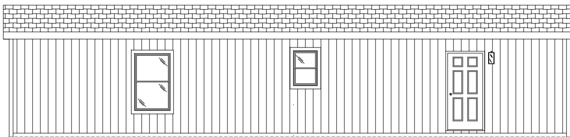
FRONT SIDEWALL
