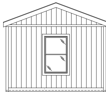
STD. FRONT ENDWALL
