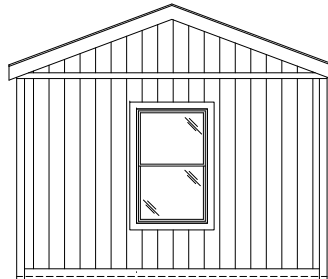
STD. FRONT ENDWALL
