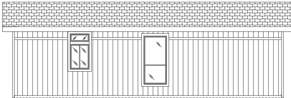
REAR SIDEWALL
