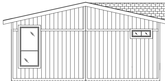
REAR ENDWALL
