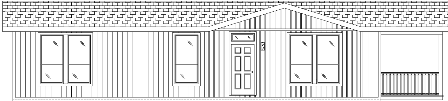
FRONT SIDEWALL W/ OPT. PORCH
