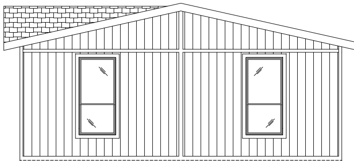
FRONT ENDWALL
