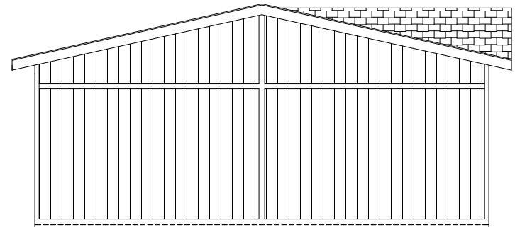
REAR ENDWALL
