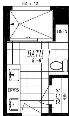
OPT. 48x72 SHWR. W. DBL LAVS
