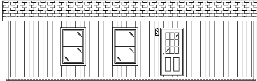
REAR SIDEWALL
