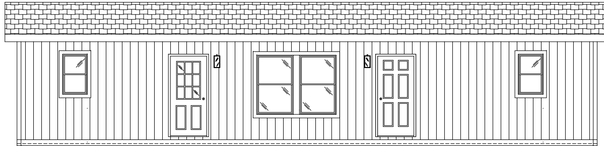
FRONT SIDEWALL
