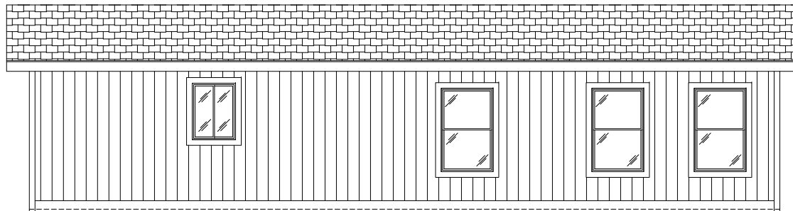
BACK SIDEWALL
