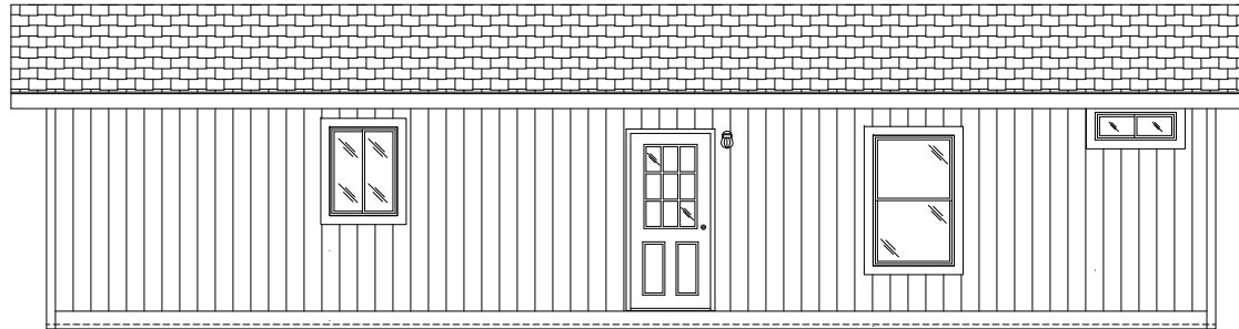
BACK SIDEWALL
