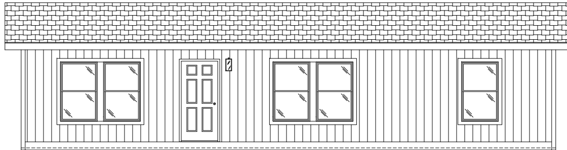
FRONT SIDEWALL
