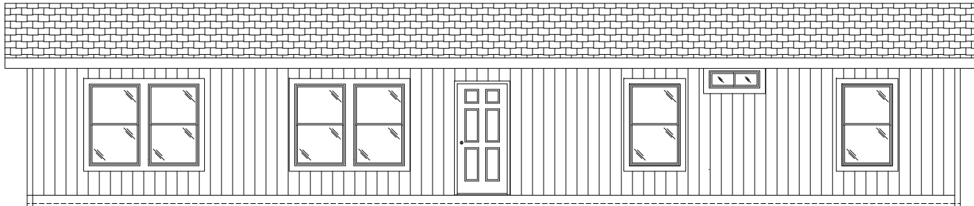
FRONT SIDEWALL
