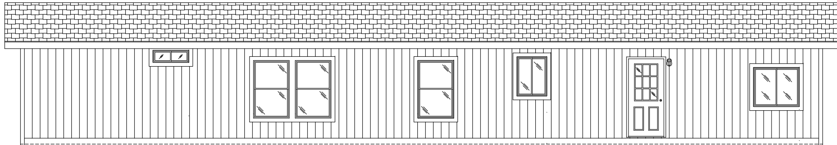
REAR SIDEWALL
