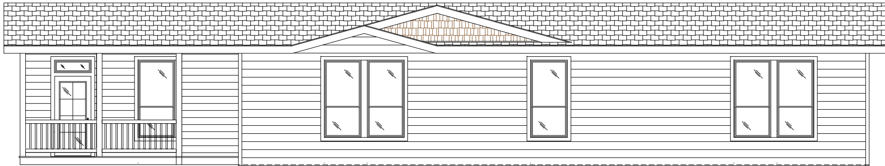
FRONT SIDEWALL
